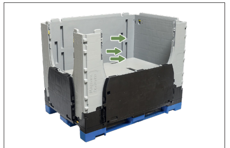
6. The internal volume of the SHP can optionally be divided into two and three areas with two divider shelves.
