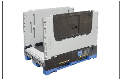
3. Erect both long sidewalls one after the other.
